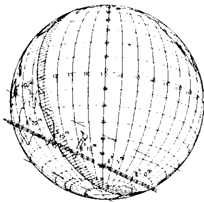
ZC 3227 by Juewa 94 Oct 8
