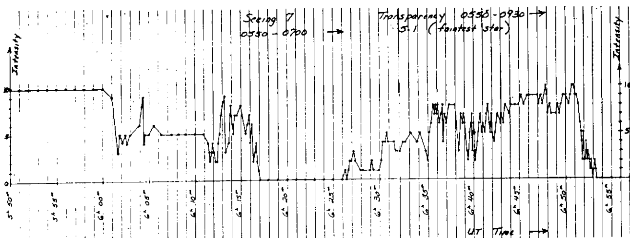
Ingress visual lightcurve, occultation of 28 Sagittarii by Saturn, 6" refractor, 350X, Bob Talaga, Tucson, AZ
