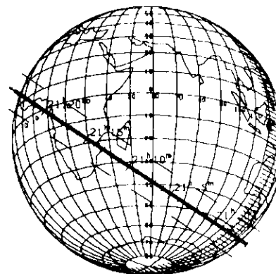
SAO 183095 by Victoria 1985 Apr 21
