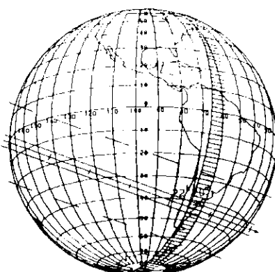
SAO 159188 by Vesta 1985 Sep 12
