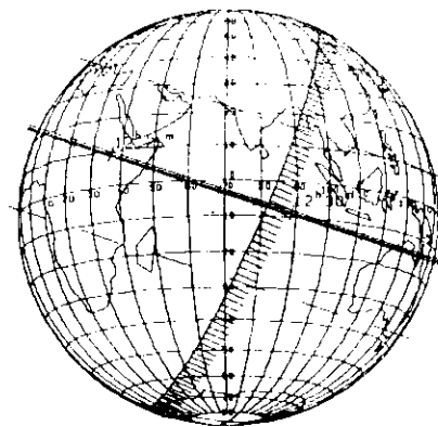
SAO 157588 by Medea 1985 Jul 17
