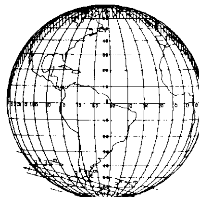
SAO 120229 by Vesta 1985 Apr 23
