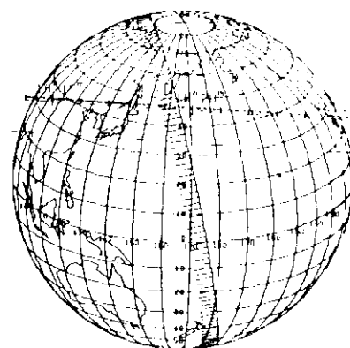
+20° 626 by Kleopatra 1985 Aug 26
