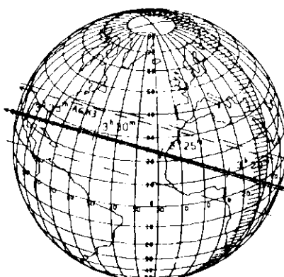
SAO 76770 by Panopaea 1985 Nov 5
