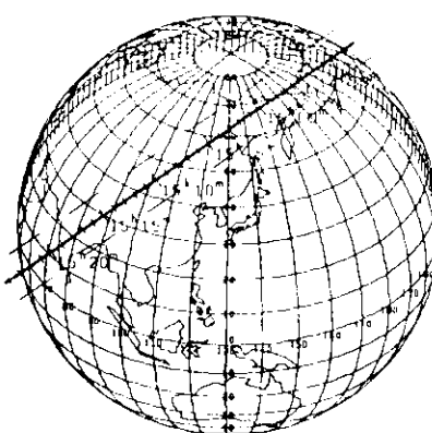
SAO 55372 by Semiramis 1985 Oct 27
