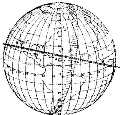
SAO 96895 by Aemilia 1985 Oct 31
