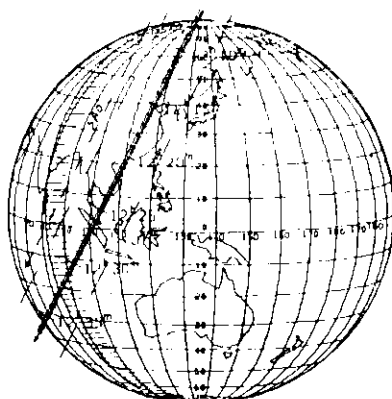
SAO 127622 by Athamantis '85 Oct 9
