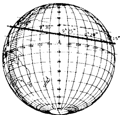
SAO 159657 by Hestia 1985 Jun 21
