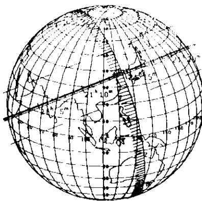
SAO 75635 by Isolda 1985 Aug 25
